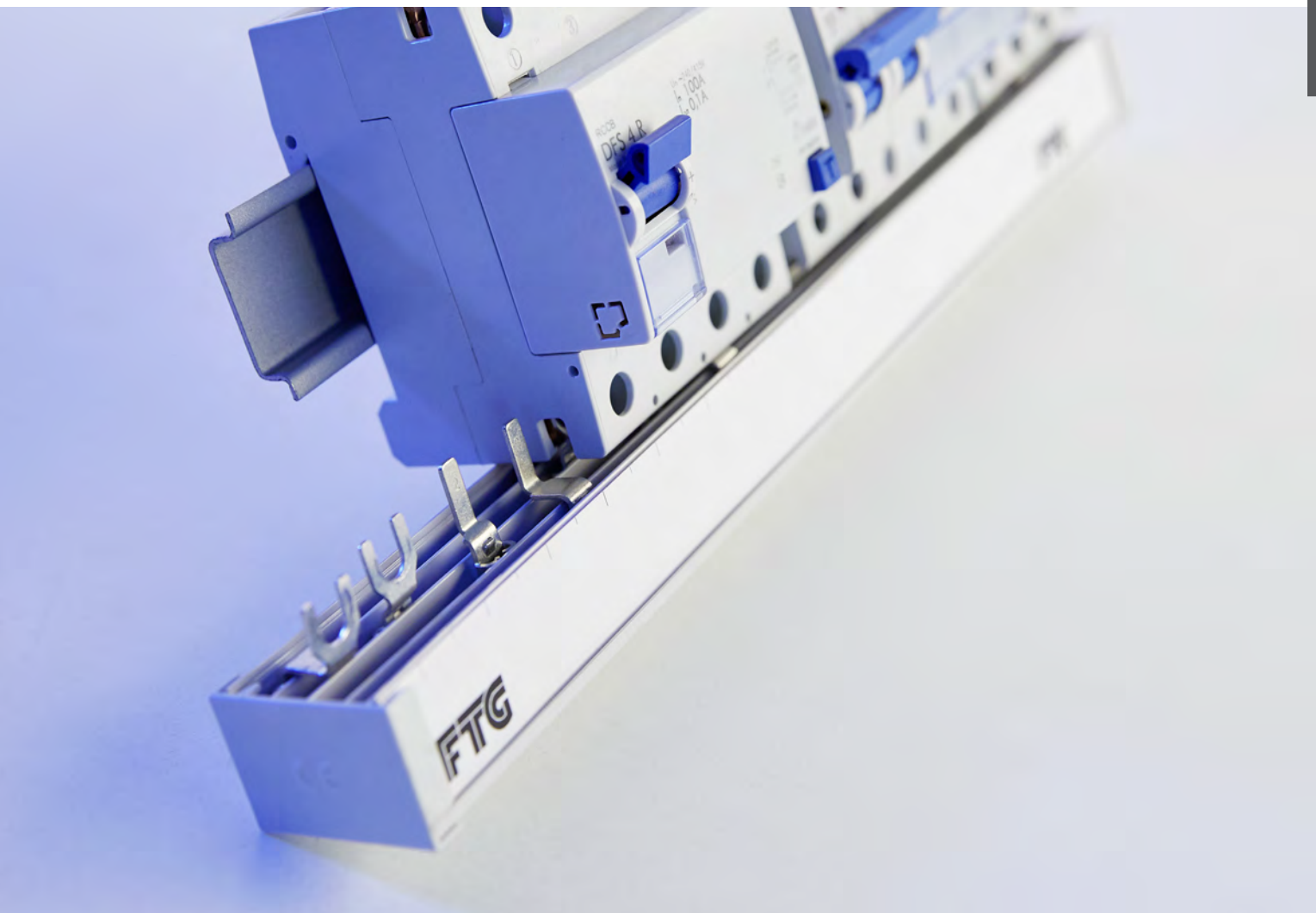
FCBeasy in Anwendung | FCBeasy in application | FCBeasy en application
